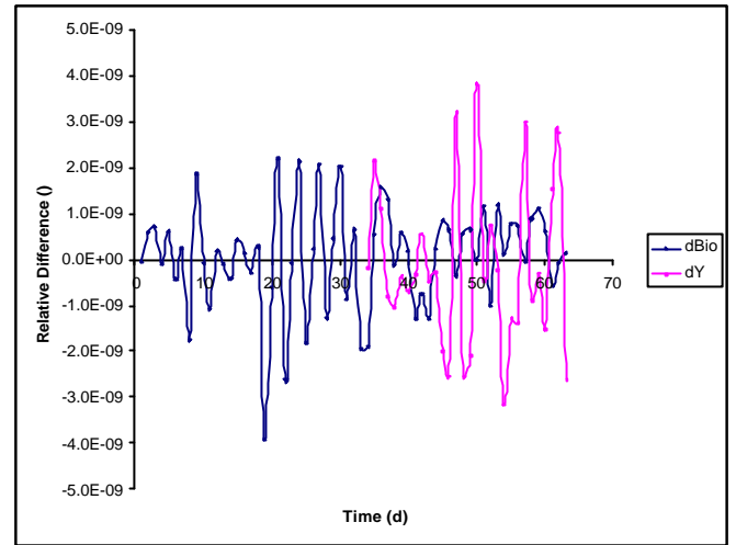
Figure 6: Wheat model Relative Differences
