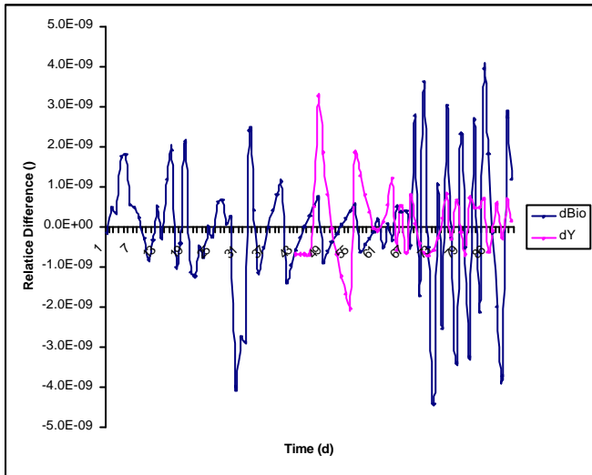
Figure 3: Tomato Model Relative Differences
