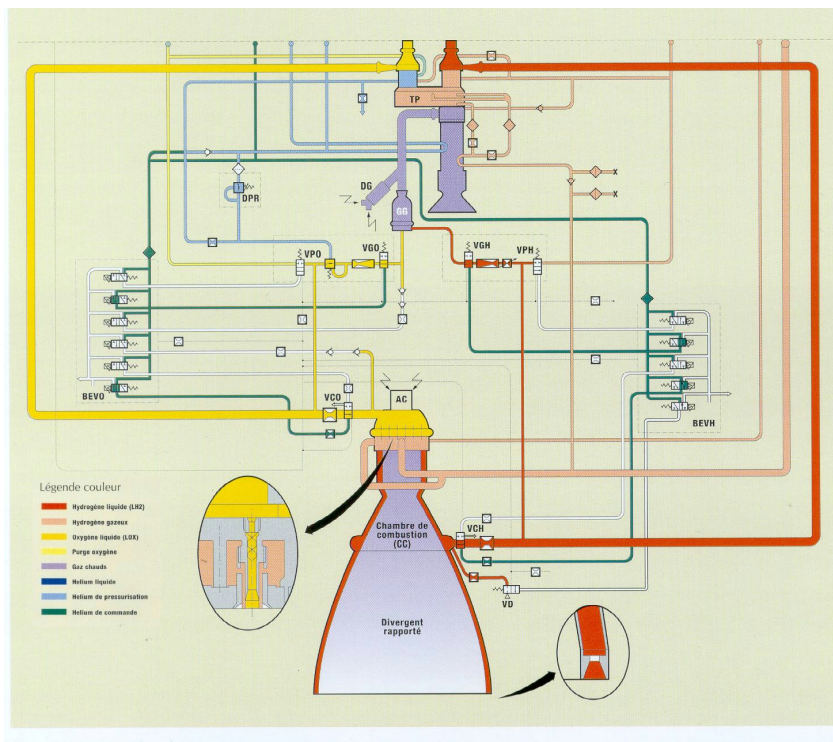
Figure II-1. HM7B engine
